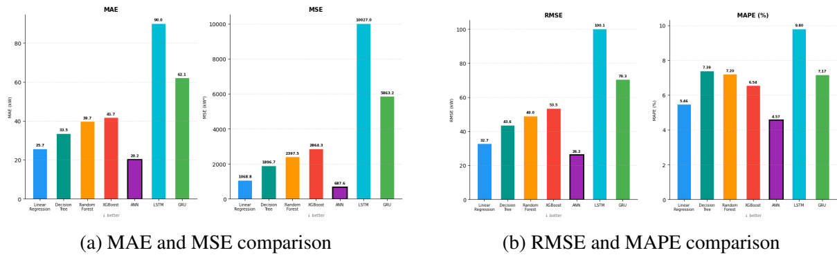
Figure 4.2: Comparative analysis of regression error metrics across the evaluated machine learning models (5-Fold CV).
