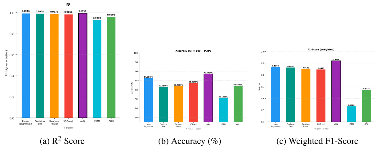
Figure 4.3: Comparative performance scores ( R^2 , Accuracy, and F1-Score) distribution for machine learning and deep learning models.
